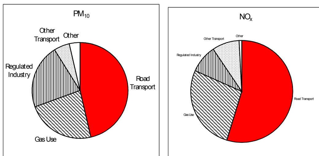
Figure 13. Proportion of emissions of \text{NO}_x and \text{PM}_{10} from different sources within Greater London in 2001
