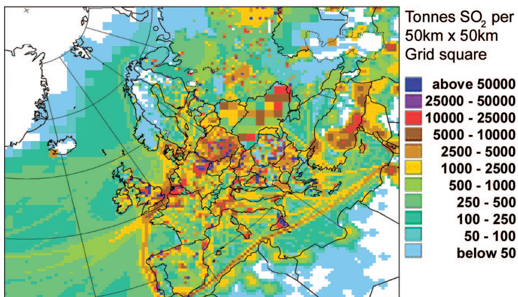
Figure 1 \text{SO}_2 emissions in Europe and the Eastern Atlantic, showing the shipping emissions in the Western Approaches to Europe, from Atlantic and in the North and Mediterranean Seas (EMEP/MS-C-W, 2001)
