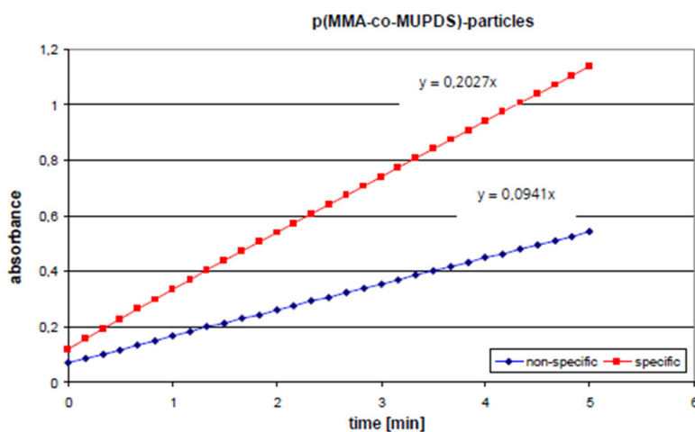
Figure 16. Measurement of enzymatic activity of particle-bound Glucose Oxidase. Both active-ester functionalised and hydrolysed particles have been investigated to differentiate between specific and non-specific binding.
