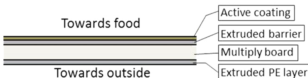
Figure 1. Example of a sandwiched packaging structure for a liquid-containing active packaging
