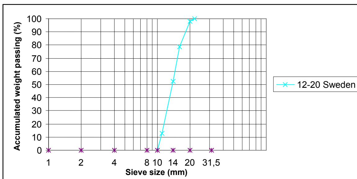
Figure 3.3 Typical grain distribution curve for LWA 12-20 produced by Optiroc in Sweden
