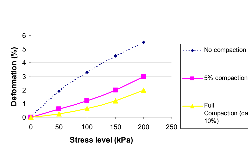
Figure 5.1 Characteristic load deformation curves, Leca ISO 10-20
