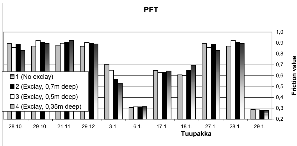
Figure 4.16 Average PFT results from Tuupakka /5/.
