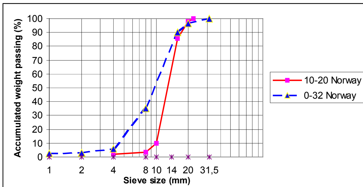
Figure 3.1 Typical grain distribution curves for LWA produced by Optiroc in Norway
