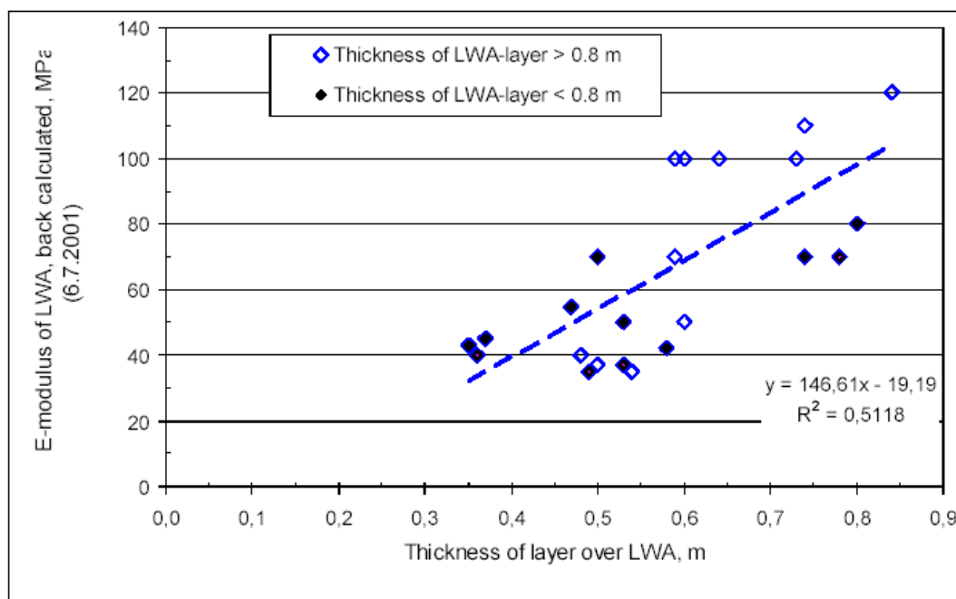
Figure 4.3 E-modulus of LWA versus thickness of cover layer
