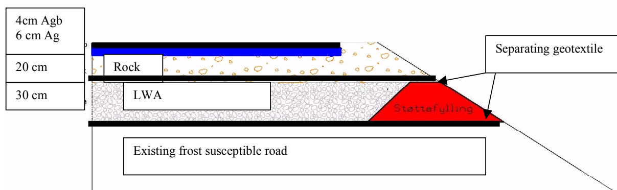
Figure 5.2 LWA as frost insulation in a road structure
