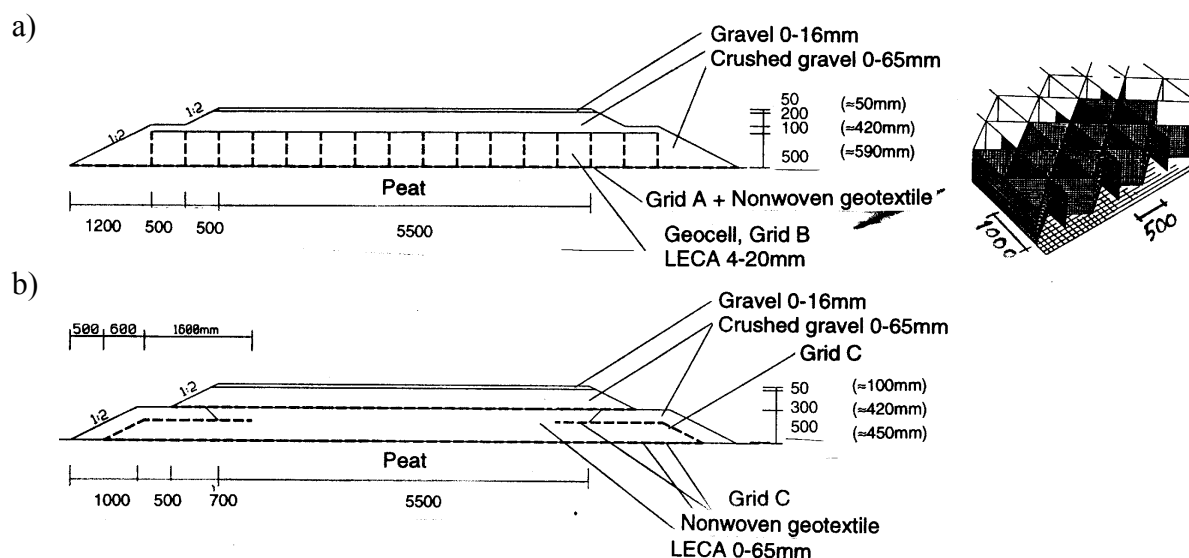
Figure 3.5 Geogrid and geocell reinforced test structures of Leteensuo peat area: (a) geocell + LWA, (b) 2 x geogrid + LWA. The fulfilled layer thickness are presented in the brackets (Finnish georeinforcement research 1990...2001) /16/.
