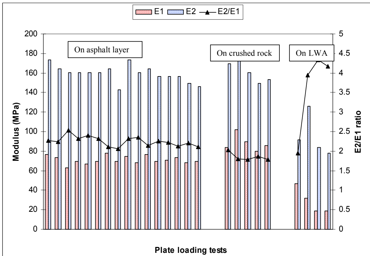
Figure 4.13 Results from plate loading tests during excavation
