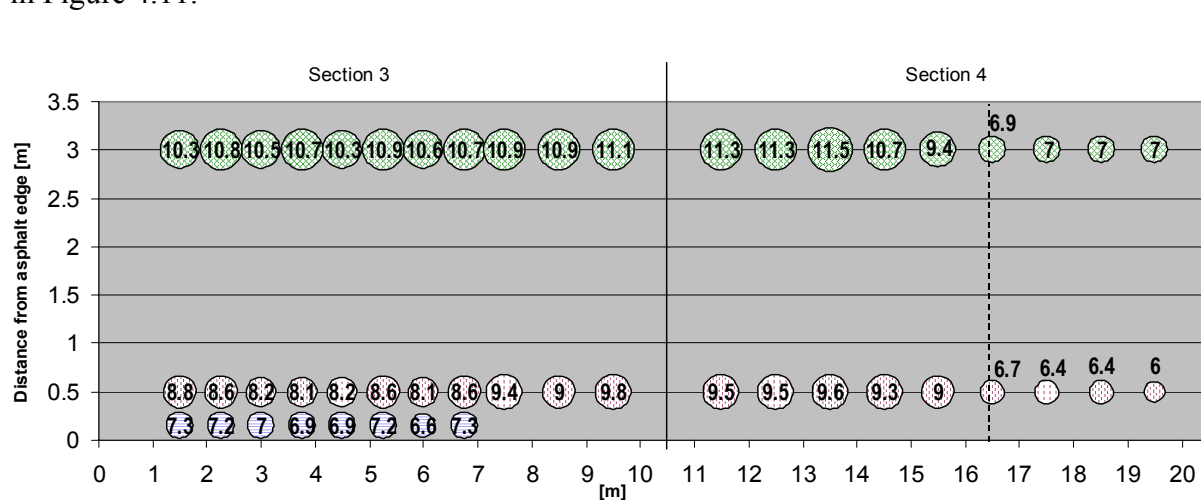
Figure 4.11 Bearing capacity (tons) measured with FWD (1 ton eq 10 kN)
