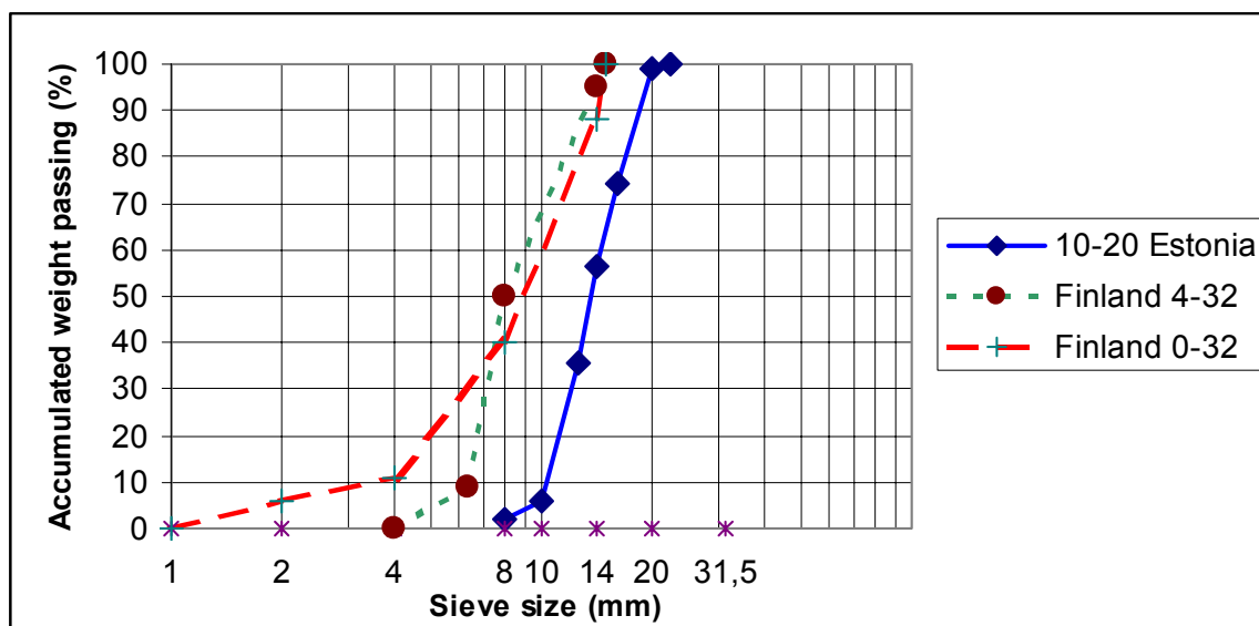
Figure 3.2 Typical grain distribution curves for LWA produced by Optiroc in Finland and Estonia
