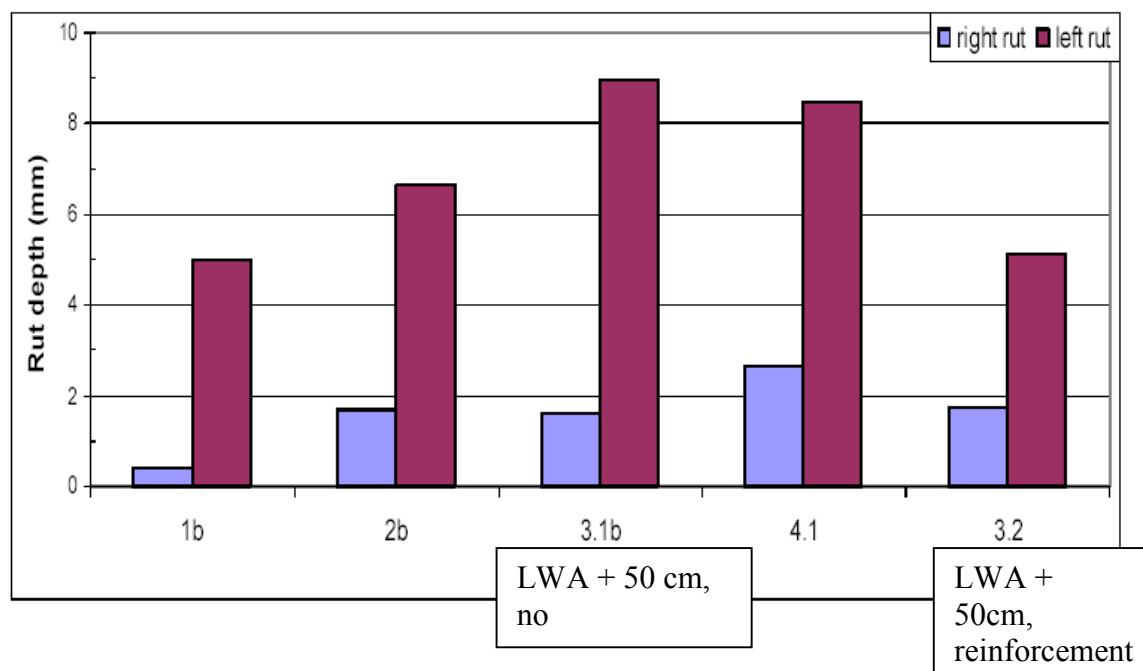
Figure 4.4 Rut depth of the test sections in Tuupakka at 2001-10-01
