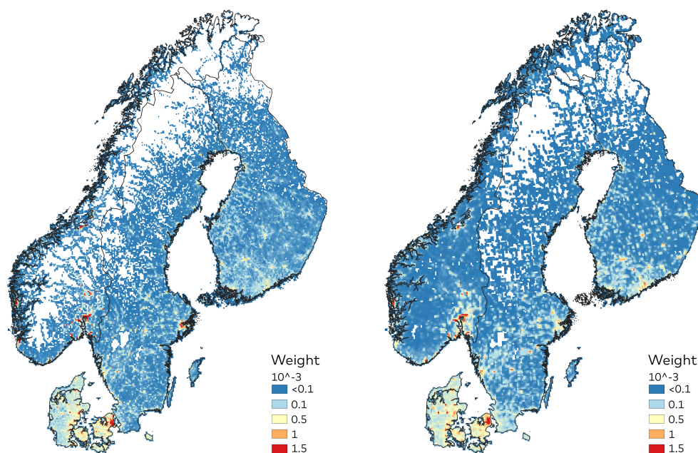
Figure 10. Normalized spatial distributions of PM 2.5 emissions from residential combustion in the NordicWelfAir-inventory (left), and from the new inventory produced in this project (right). Normalization of the emissions were done separately for each country.
