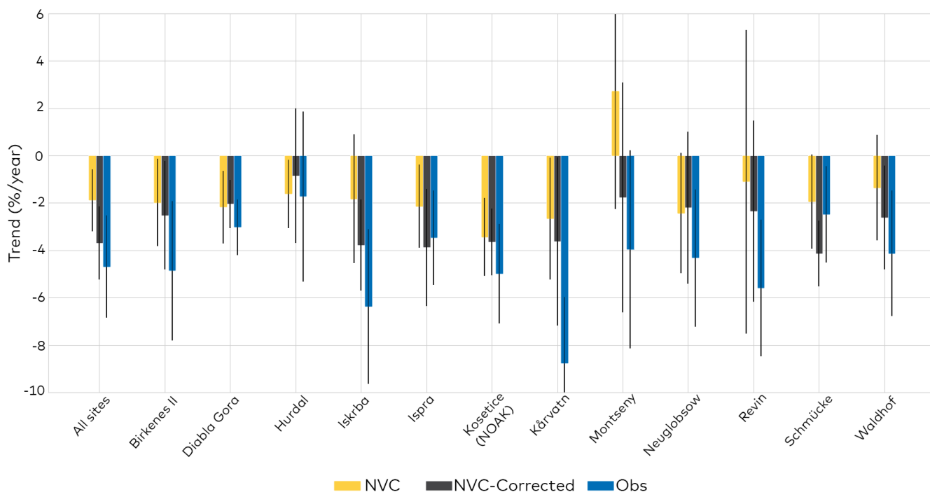
Figure 21. 2010–2019 trends for PM 2.5 (DJF) at all sites that have both PM 2.5 and OC 2.5 measurements, for observations, NVC and NVC-Corrected. For single stations, uncertainty bars represent the standard deviation ( \sigma ) of the mean of the trends.
