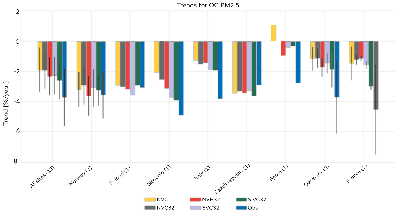
Figure 18. Comparison of calculated DJF trends over 2010–2019 with five model scenarios, compared to measurements. Numbers in brackets give the number of sites. Here, the trends give the average of the individual trends calculated for each site, and error bars indicate the standard deviation ( \sigma ) among sites where relevant.
