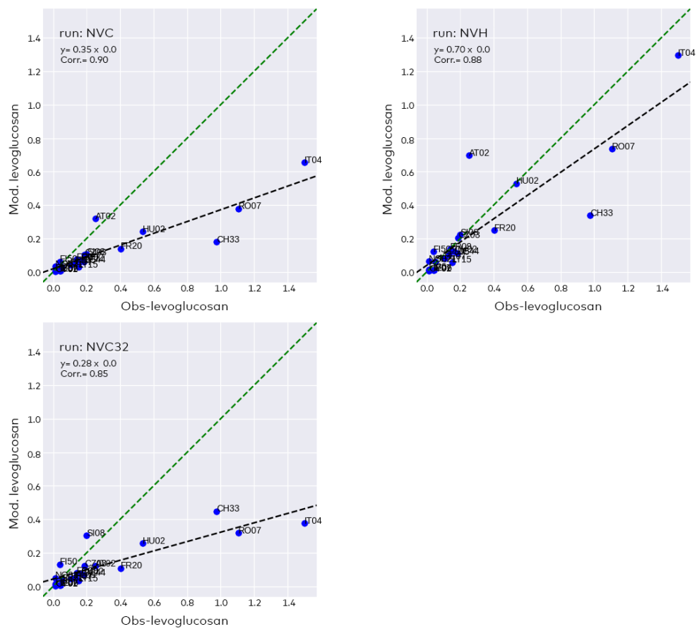
Figure 14. As Fig. 13, but for levoglucosan.
