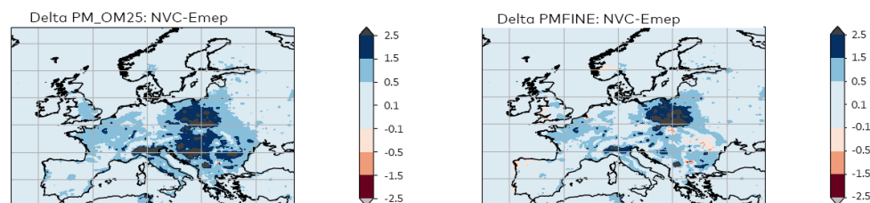
Figure 23. Deltas ( \mu\text{g m}^{-3} ) of \text{OM}_{2.5} (left) and \text{PM}_{2.5} (right) from Ref2 v2.1 scenarios compared to EMEP.
