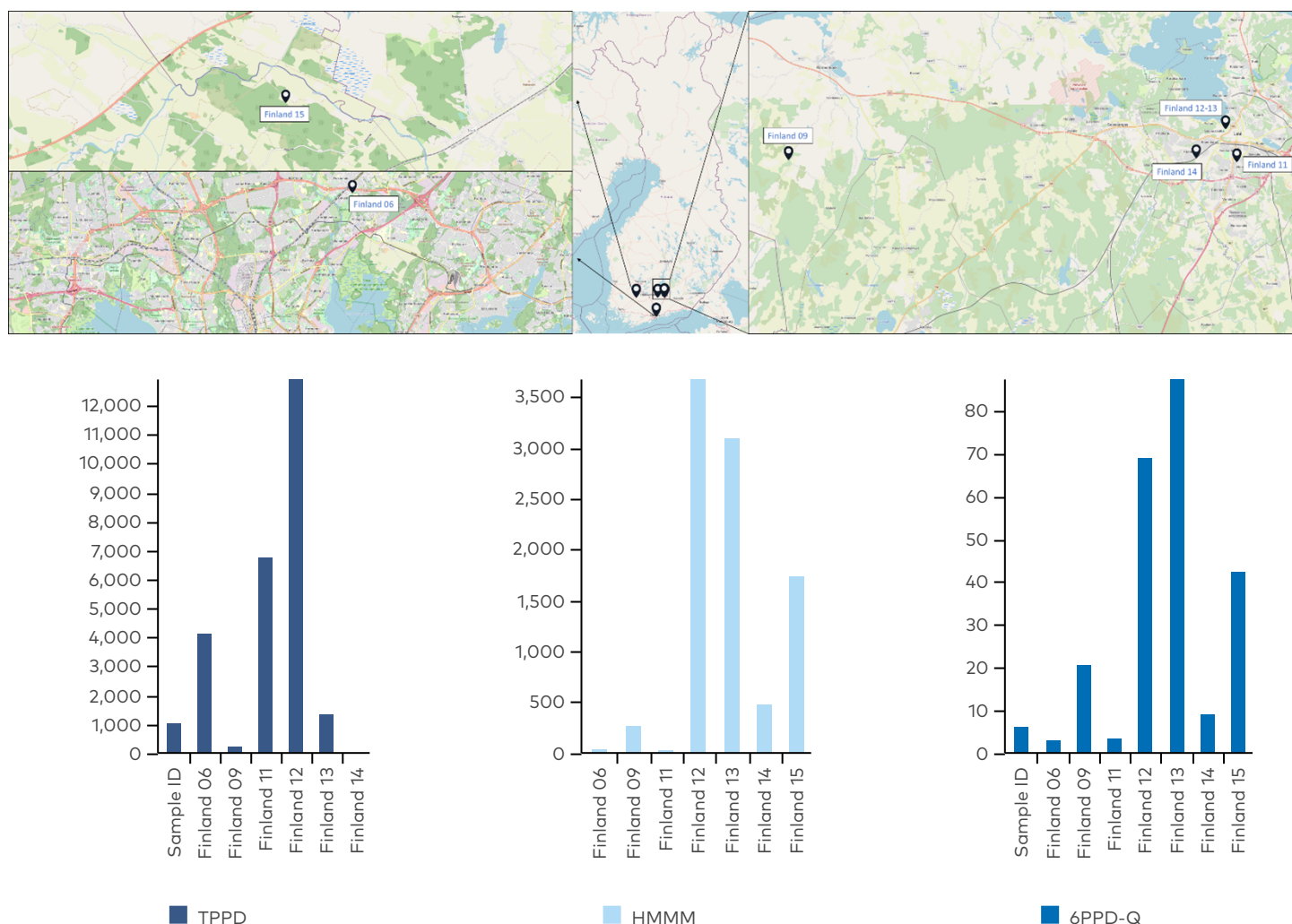
Figure 8: Concentrations in ng/L of selected tire related additive chemicals detected in water samples from Finland.
