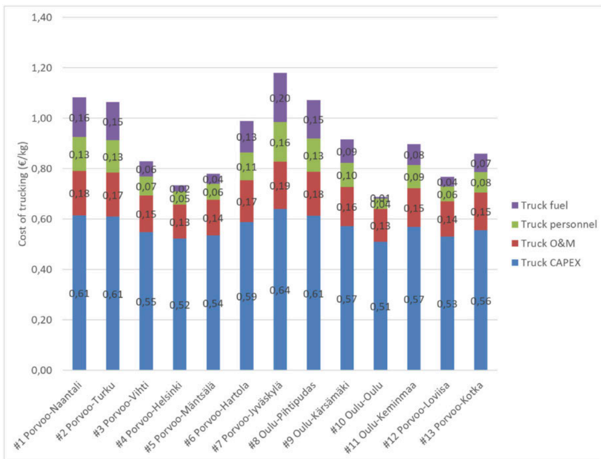
Figure 6. Trucking cost for hydrogen in Finland for selected routes. Each station processes 1,000 kg/day. Hydrogen payload 1,500 kg/truck. Truck CAPEX includes hydrogen containers.
