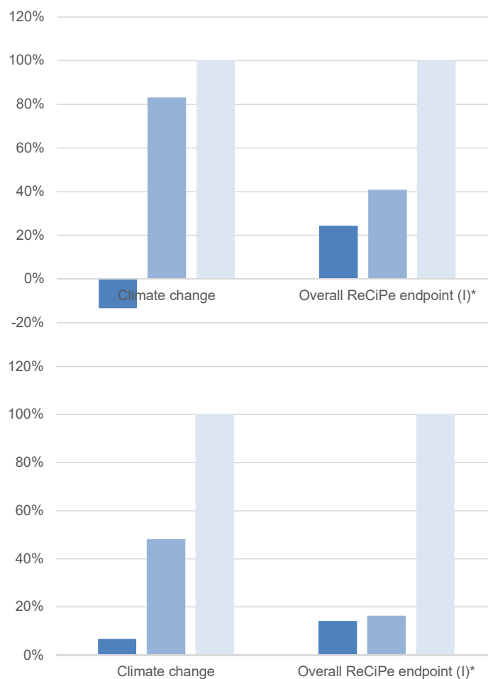
< Figure 76 RELATIVE RESULTS FOR roof tile CASE VS ALTERNATIVES, INCLUDING AVOIDED EMISSIONS FROM SUBSTITUTION (TOP), EXCLUDING AVOIDED EMISSIONS (BOTTOM).
